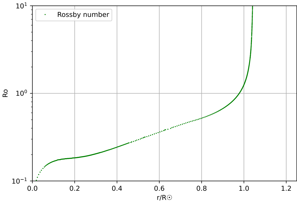
Rossby number, profile 153, age 6.01 \times 10^9
